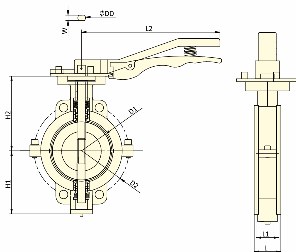
SECTIONAL VIEW
