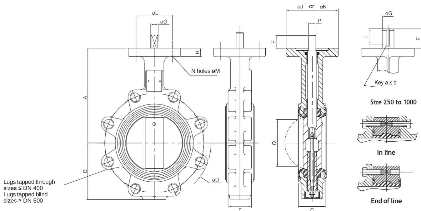
VALVE DIMENSIONS (mm)
